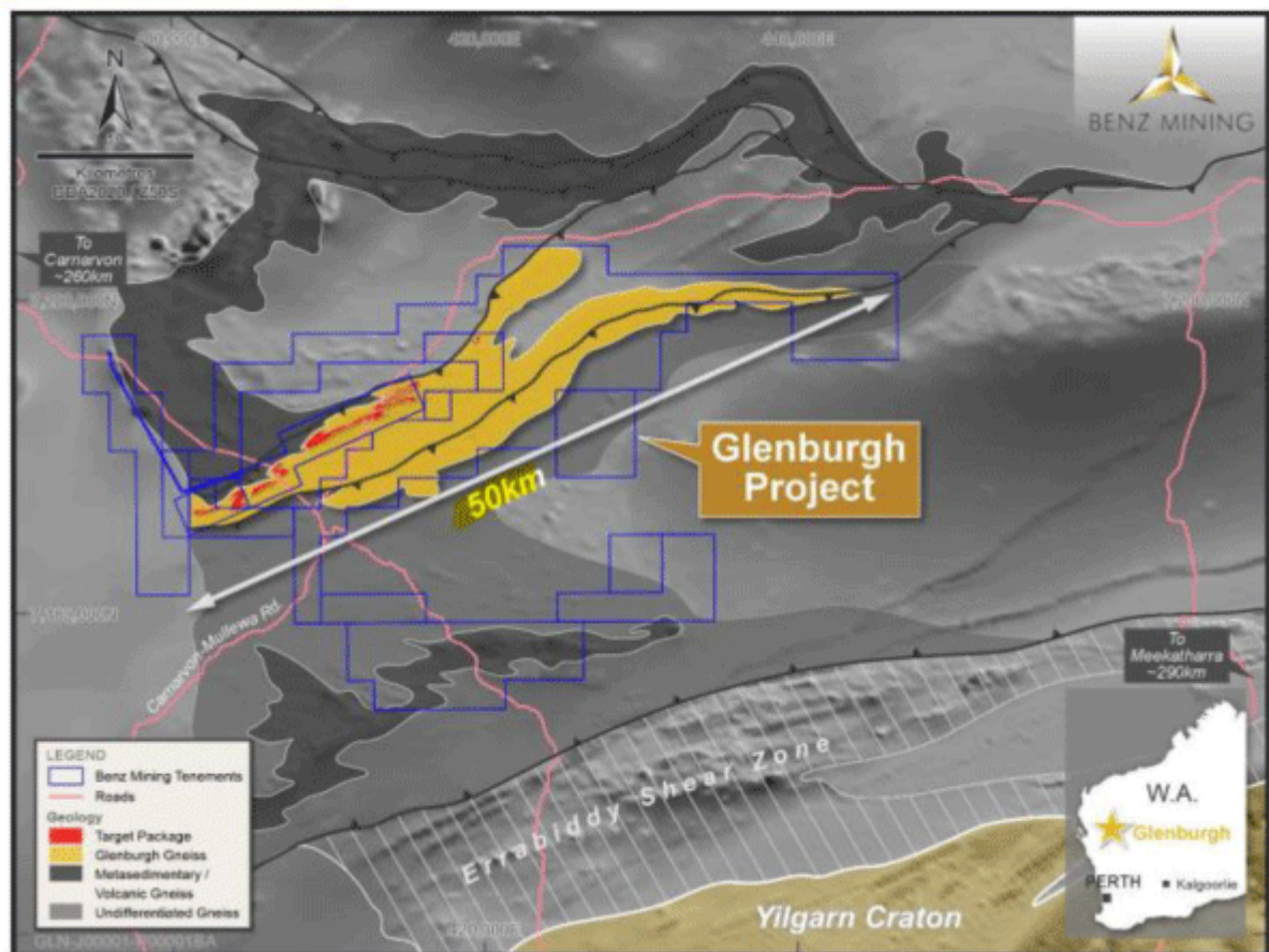
Figure 2: Geology overview of the Glenburgh Project
