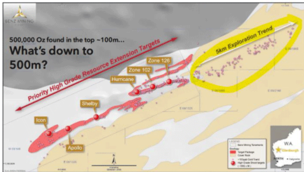
Figure 3: Detailed geological map of the Glenburgh Project
