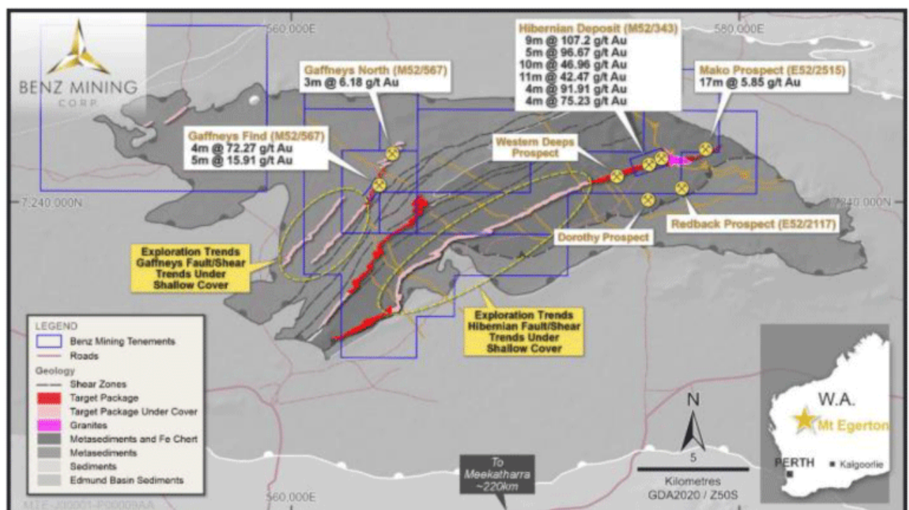
Figure 6: Mt Egerton Project geology overview
