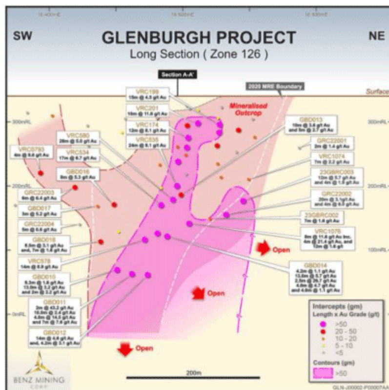
Figure 4: Long section of Zone 126 at Glenburgh Project
