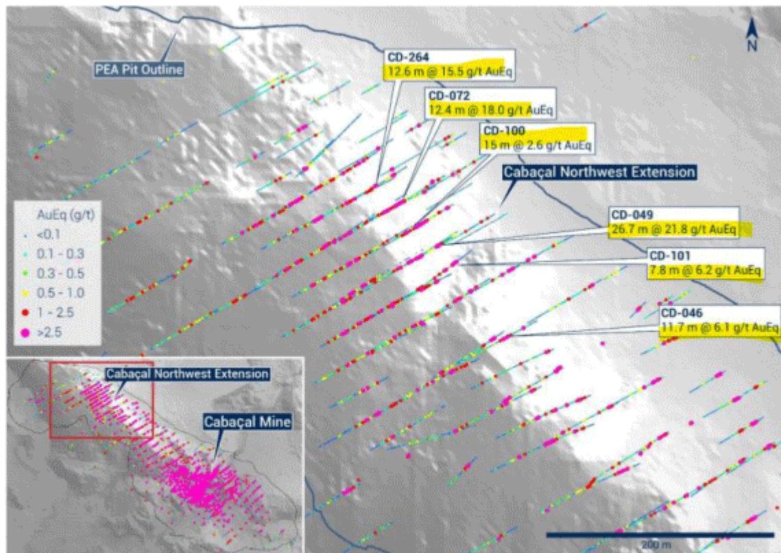
Figure 1: Location of CD-264's intersection, extending the projection of the high-grade CNWE trend. Colour points represent drill assays plotted as AuEq (g/t) in plan view. Digital elevation image in the background.
