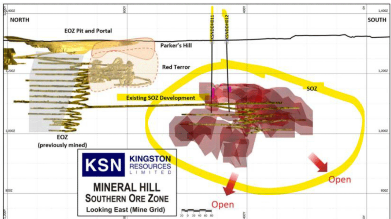
Figure 2: Long section looking east at SOZ with KSNDH011 and KSNDH012.
