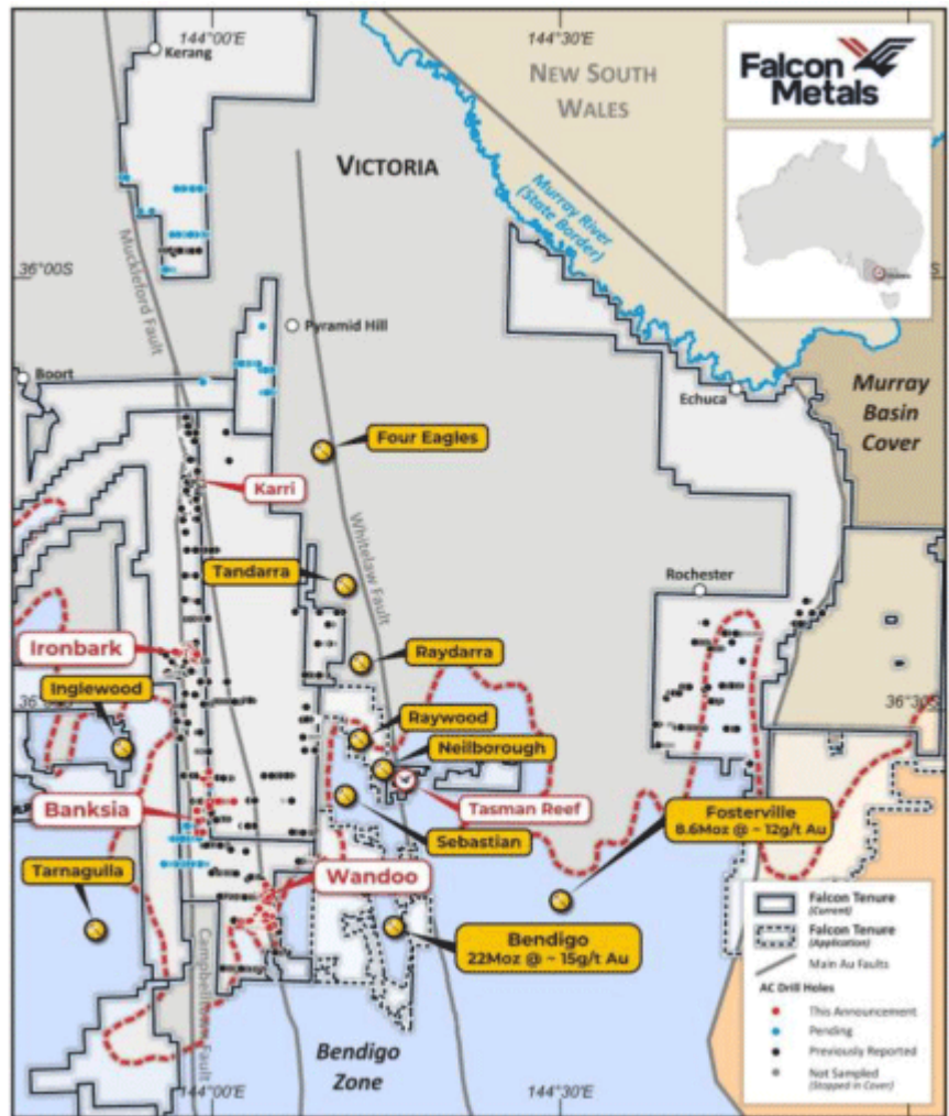
Figure 1 Plan map showing aircore drilling status for the Pyramid Hill Gold Project
