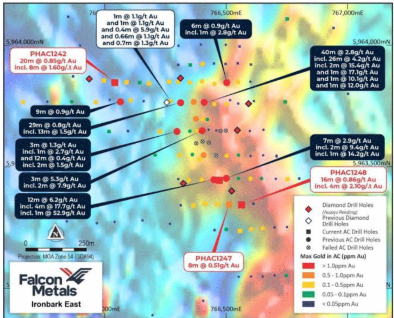
Figure 5 Inset Plan map from Fig. 4 of Ironbark East showing new aircore results
