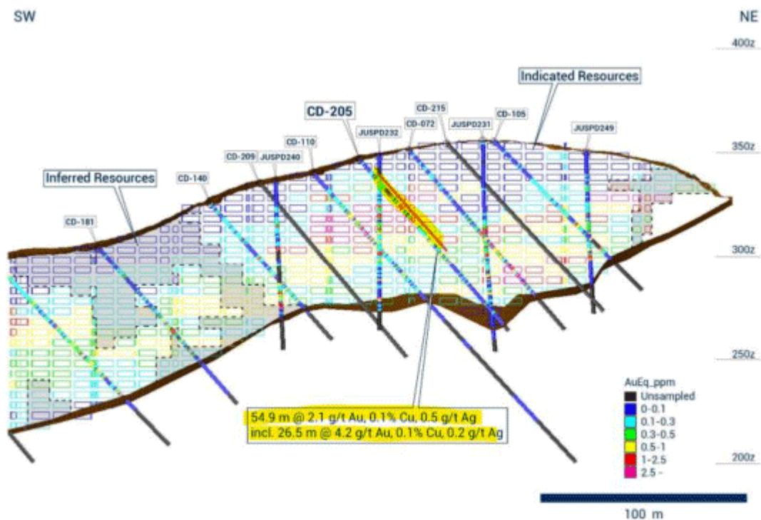
Figure 2: Cross section A - A' through the CNWE's shallow high-grade zone (view to the northwest; refer to Figure 1 for location).
