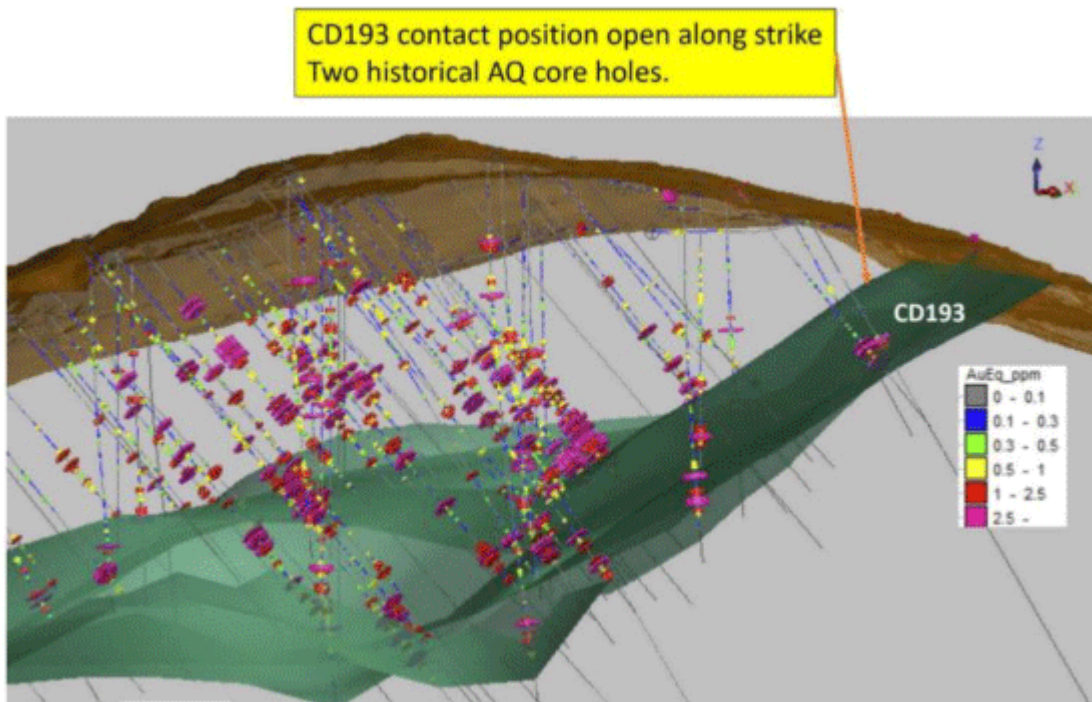
Figure 3: 500m window with hole traces coloured by gold-equivalent, showing the open contact along strike from CD193 (view to the northwest).
