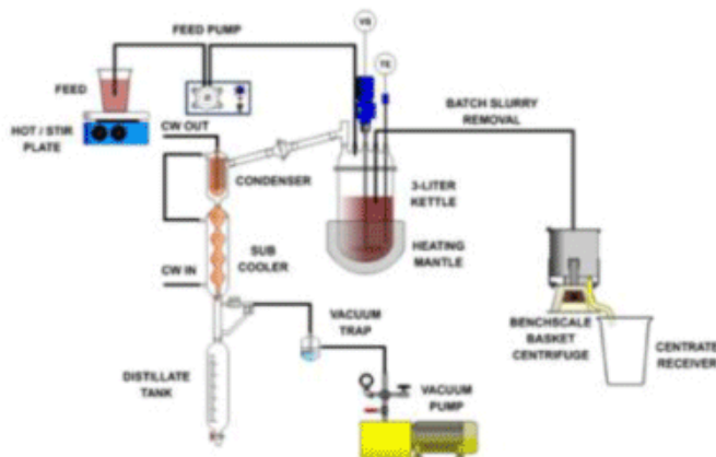
Figure 2. Schematic crystallisation bulk test programme flowsheet design.
