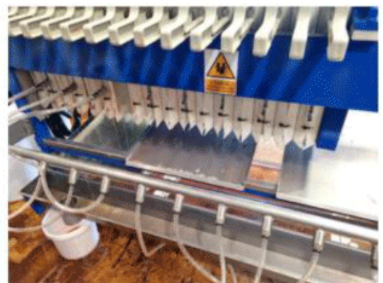
Figure 3. Laboratory test equipment in operation.
