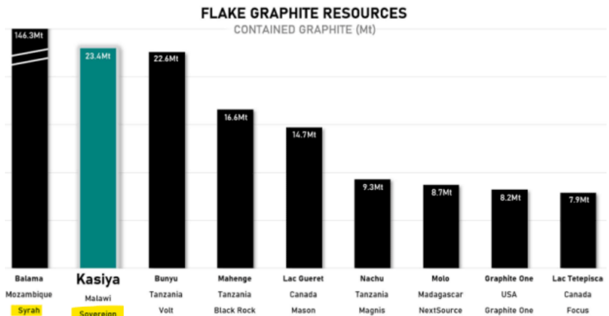
Figure 2: Major listed global flake graphite resources (Sources: refer to Appendix 1)
