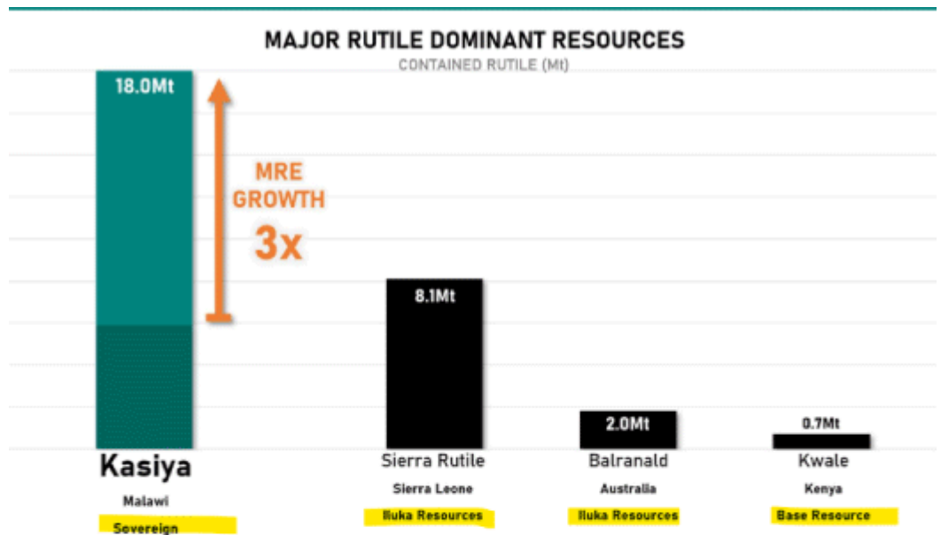
Figure 1: Major rutile dominant resources (Sources: refer to Appendix 1)
