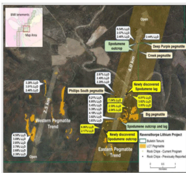
Figure 1: Spodumene locations, LCT pegmatite locations and rock chip assays above 2.0% Li 2 O with new results highlighted in yellow (refer ASX announcements dated 24 January 2022, 17 & 21 February 2022 and 21 March 2022)
