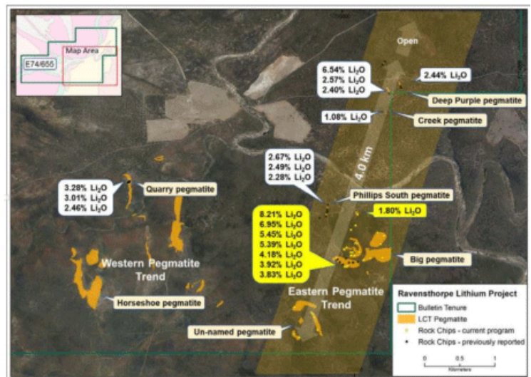
Figure 1: LCT pegmatites and rock chip assays above 1.0% Li 2 O. New results highlighted in yellow with previously reported results highlighted in white (refer ASX announcement dated 13 December 2021)
