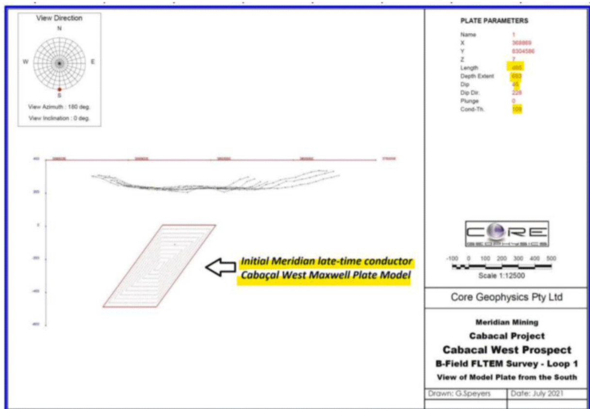
Figure 1: Top: plan view Cabacal West Conductive Response, Bottom: Modelled late-time Maxwell plate.
