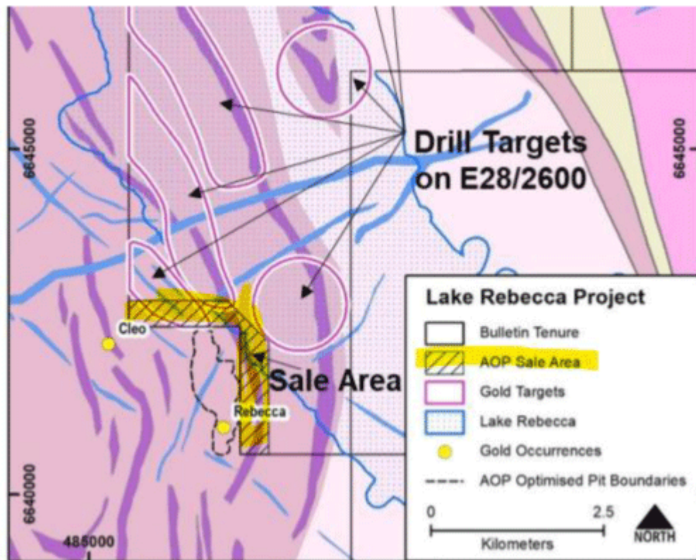
Figure 1: Sale area and priority gold targets for drilling on Lake Rebecca
