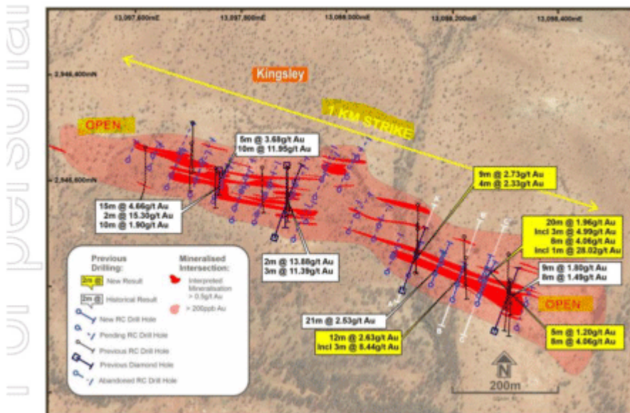
Figure 1: Kingsley Prospect showing strike extent of interpreted mineralised trends and drilling with significant intercepts
