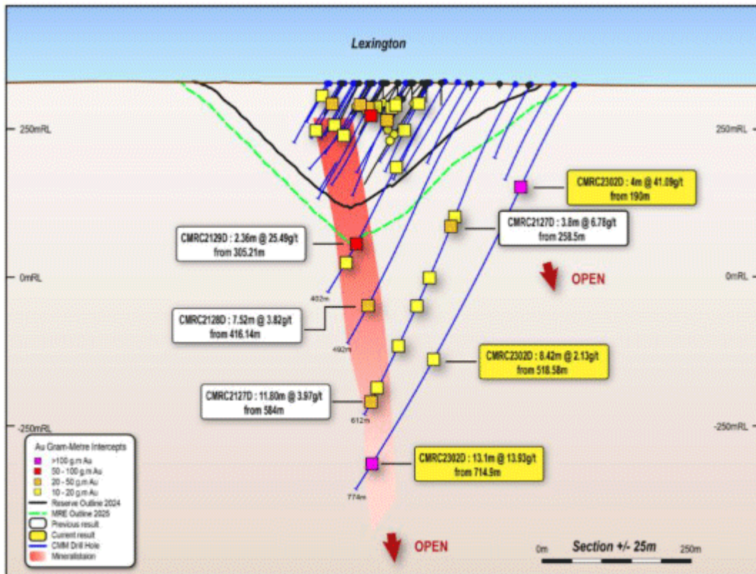
Figure 4 - Lexington section with completed diamond drilling with significant high-grade mineralisation of the primary orebody extending +400m down dip of the A$2,200/oz reserve outline with grade and thickness increasing at depth.
