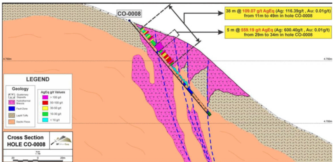
Figure 2: Geological cross-section of the Pocañita Chica Target displaying interpreted structural controls on mineralization along the drill hole trajectory and the corresponding mineralized intercept in DDH CO-0008.
