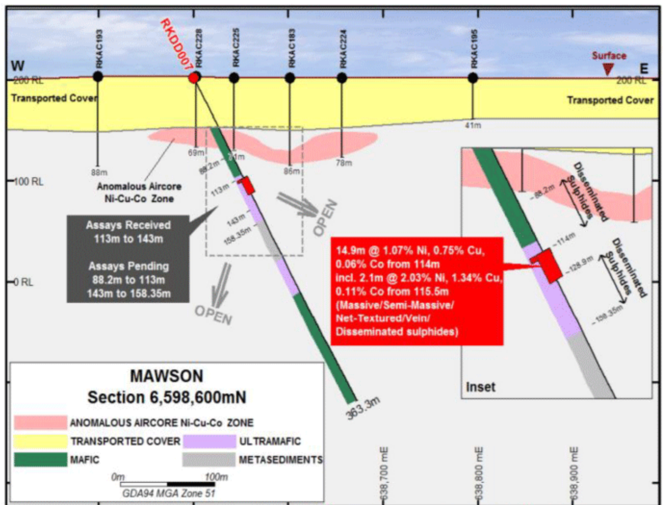
Figure 2: Drill Section 6,598,600N with Diamond Drillhole RKDD007
