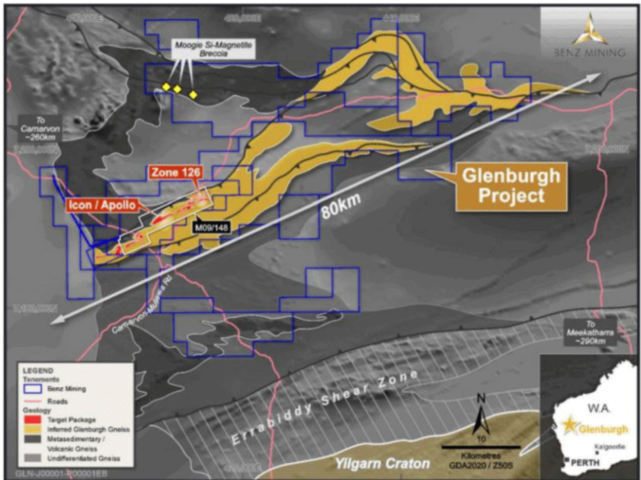
Figure 3. Geological overview of the Glenburgh Gold Project.
