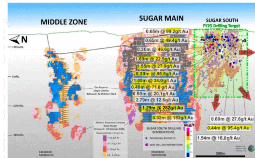
Figure 8: Sugar Zone long section highlighting emerging Sugar South target area with highlights from recent drilling
