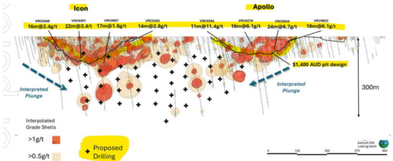
Figure 1 East West Long section view looking North of Icon Apollo with interpolated grade shells at 1g/t and 0.5g/t gold. Proposed drilling demarcated by black crosses. Previous results released on 6 November 2024 and 3 April 2025.
