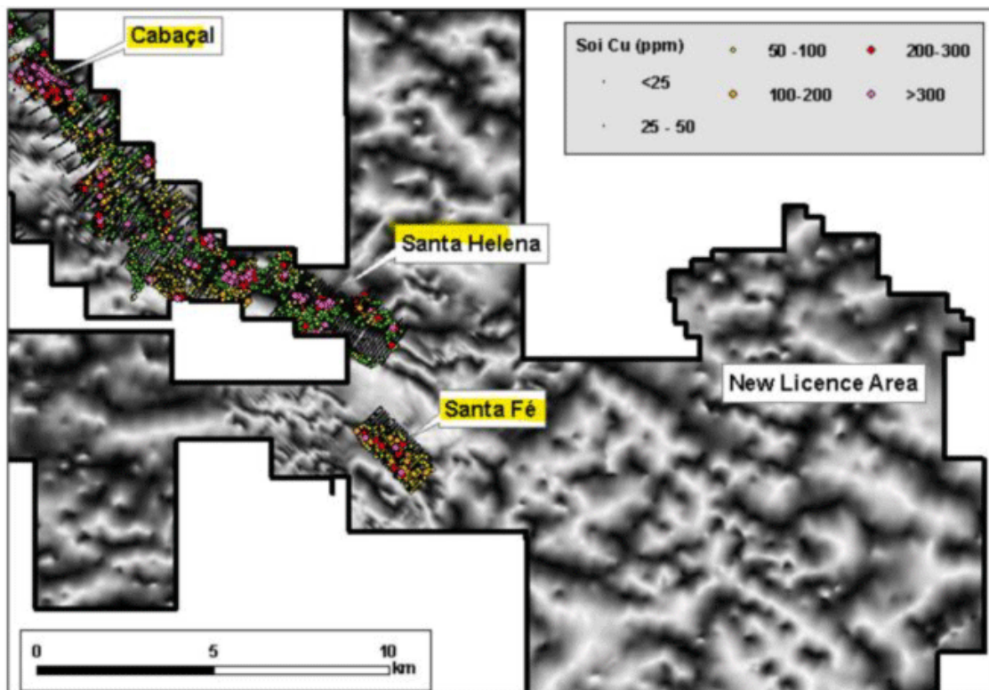
Figure 3: Newly located soil anomaly at Santa Fé, ~5km southeast of Santa Helena, marking a potential fold-repeat of the VMS stratigraphic horizon. Background image is RTP tilt-derivative magnetics.
