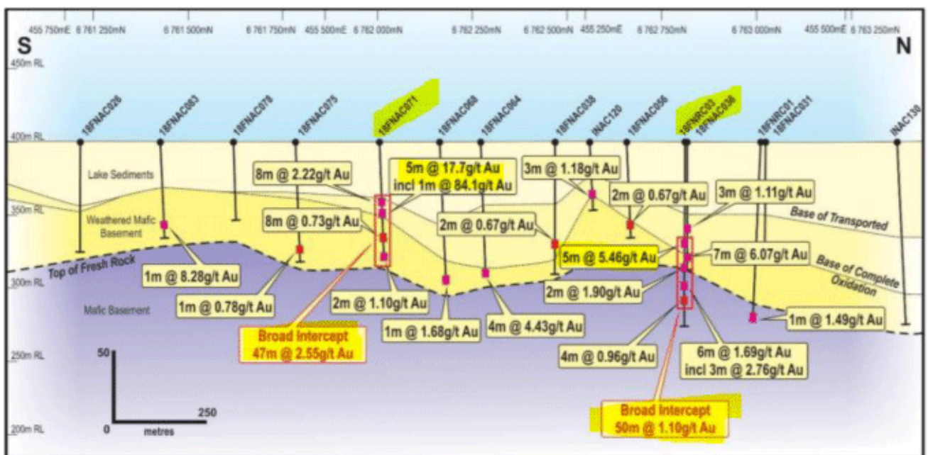
Figure 2: Fortitude North Interpreted Oblique Longitudinal Section
