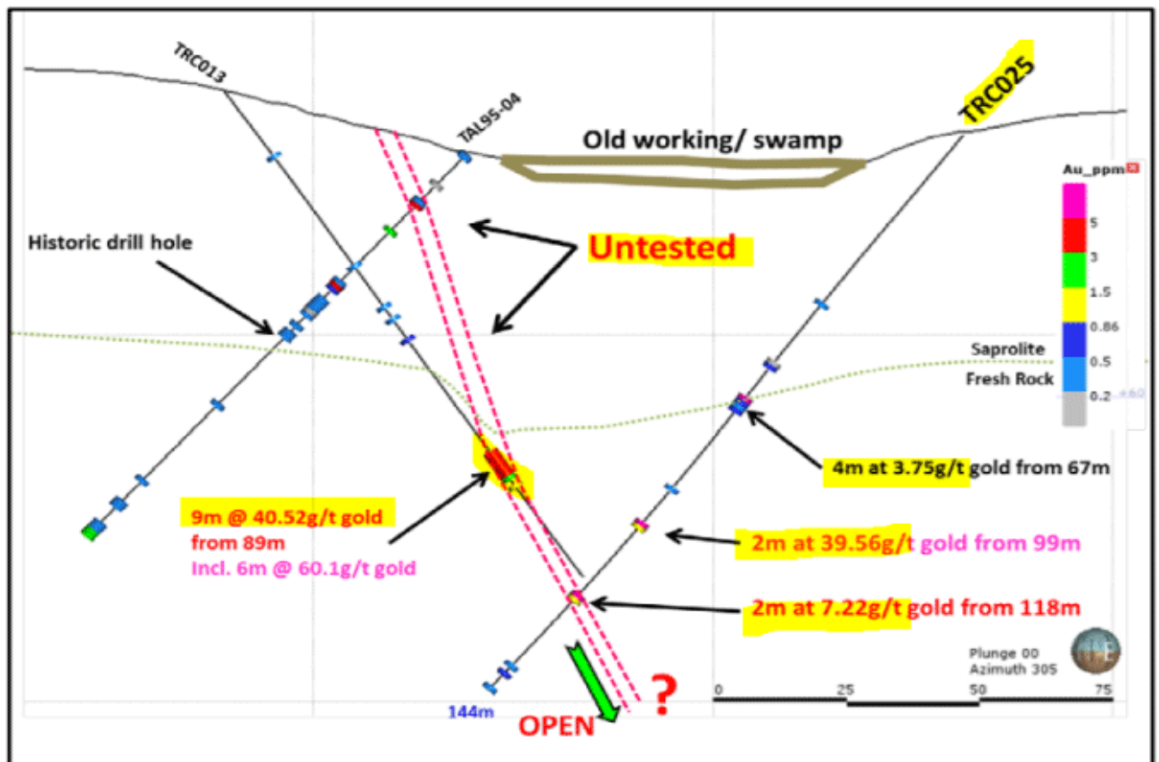
Figure 3 – Cross section illustrating key assay results from TRC013 and TRC025, as well as current preliminary geological interpretation.
