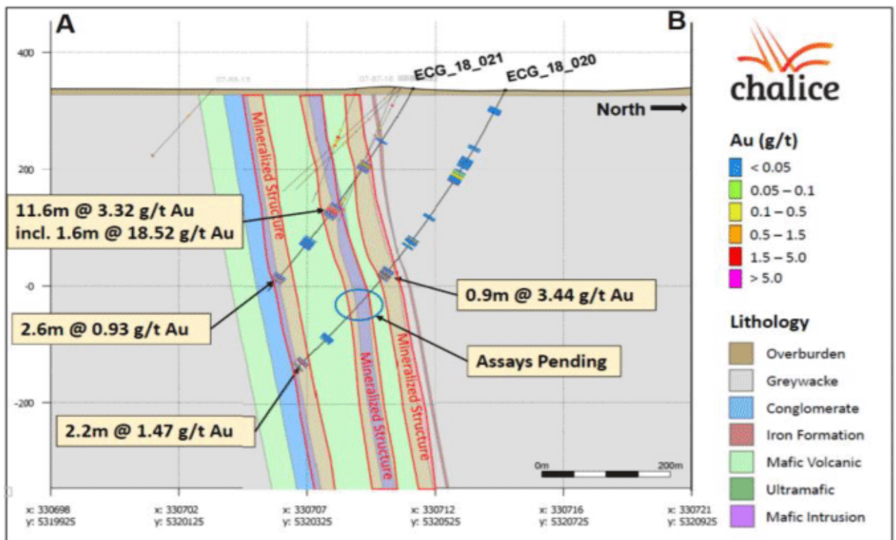
Figure 2. Simon West cross-section at drill holes ECG-18-20 and ECG-18-21.
