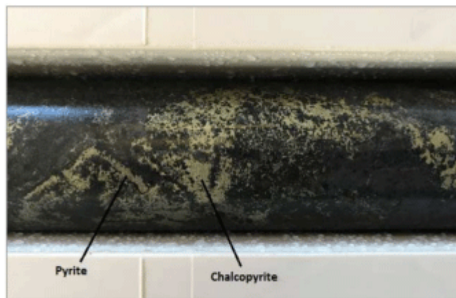
Figure 4. Interstitial chalcopryrite mineralisation, diamond drill hole WND17-001 – 255.7m depth.
