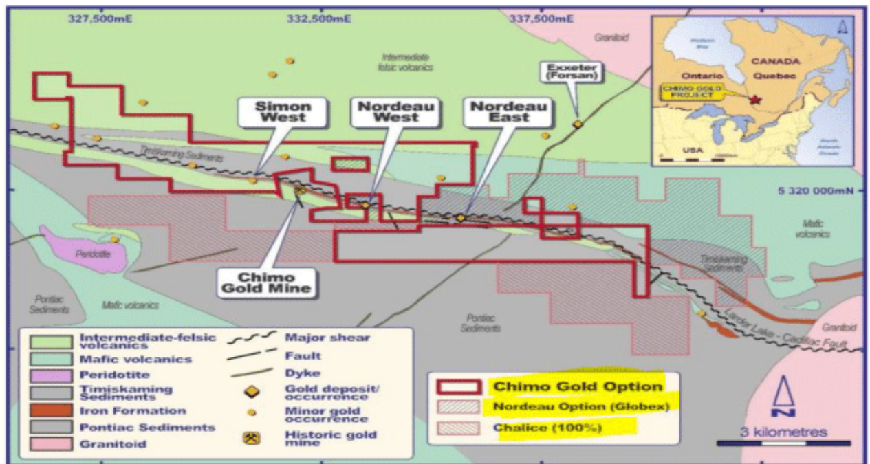
Figure 2. Local geology and tenure of the Chimo Gold Project. Existing tenure shown for the Nordeau Gold project and other claims held 100% by Chalice.
