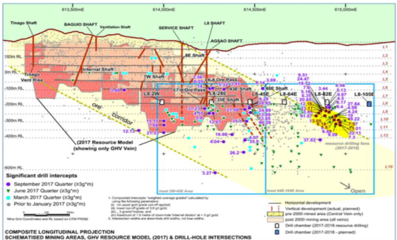
Figure 4. Co-O Mine Longitudinal Projection showing composited mining depletion, vertical development, Ore Reserves limits, and significant drill intercept locations (including previously reported). Note that the ore reserve limits are updated with the 2017 Resource Model.
